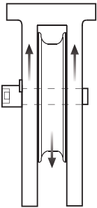
SHEAVE/PULLEY LOAD PINS (EQUALIZER/IDLER SHEAVE)
